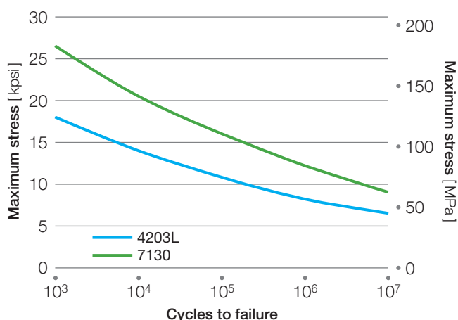
Figure 14: Tension/tension low cycle fatigue strength of Torlon® 7130 at 2 Hz, A ratio: 0.90
